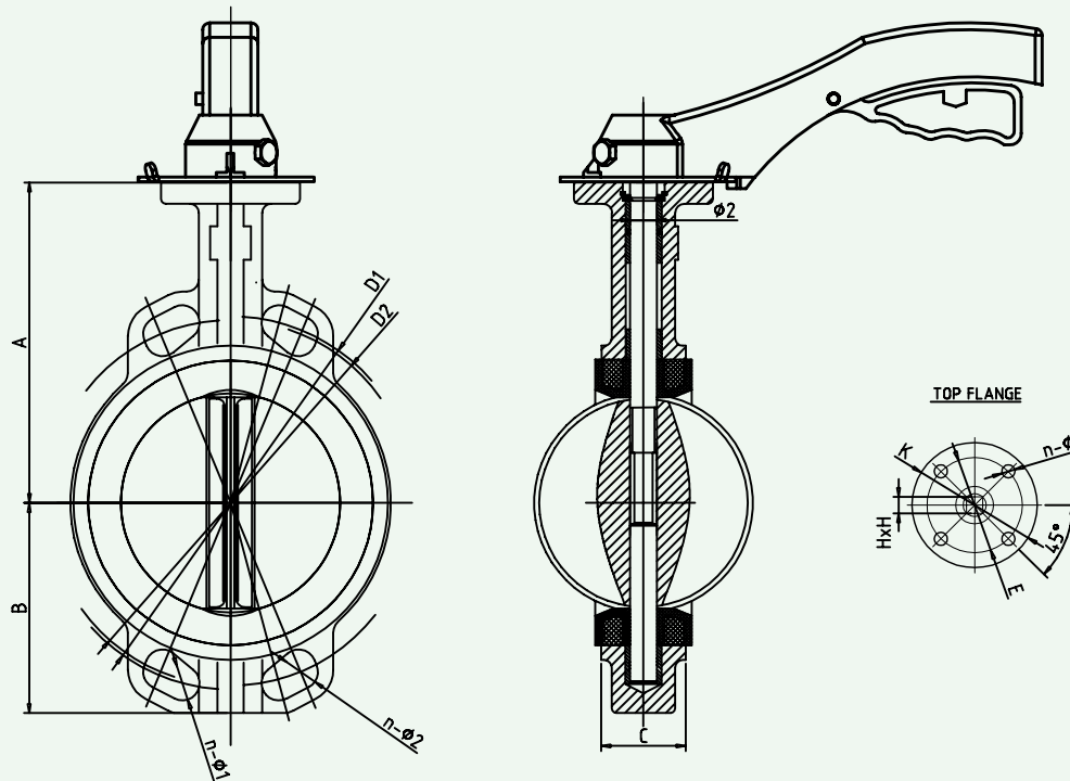
OUTLINE DIMENSIONS
